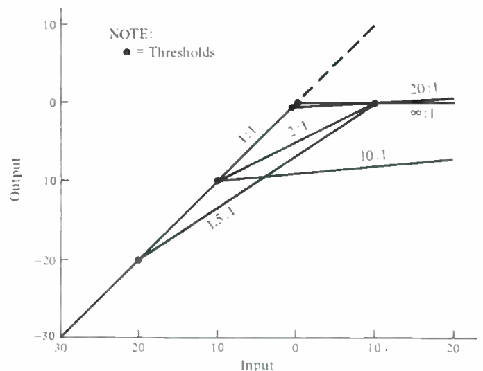
Figure 2. Typical compression and limiting slopes.
